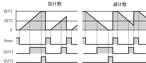
方式4 OUT2:输出保持,计数保持 OUT1:输出保持
