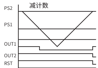
方式8 OUT1:计数值 ≥ SET1 OUT2:计数值 ≥ SET2
