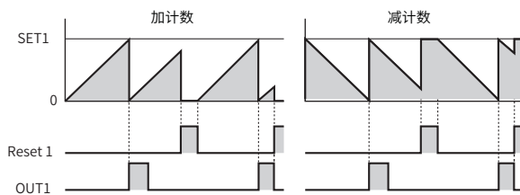
方式3/6/9 OUT1脉冲输出/计数继续
