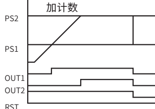
方式4 OUT1:输出保持 OUT2:输出保持, 计数保持
