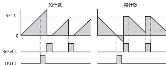
方式3/6/9 OUT1脉冲输出/计数继续
