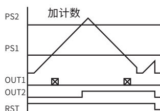
方式5 OUT1:脉冲输出 OUT2:输出保持, 计数继续
