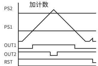
方式7 OUT1:计数值 ≥ SET1 OUT2:计数值 ≤ SET2
