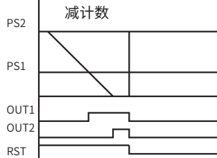
方式5 OUT1:脉冲输出 OUT2:输出保持, 计数继续
