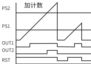
方式1 OUT1:输出保持 OUT2:输出保持, 计数继续
