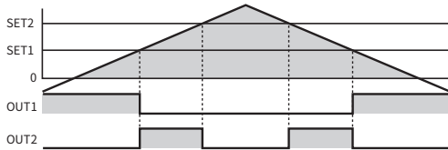
方式9 OUT1:计数值 ≤ SET1 OUT2:SET1 ≤ 计数值 ≤ SET2
