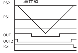
方式9 OUT1:计数值 ≤ SET1 OUT2:SET1 ≤ 计数值 ≤ SET2
