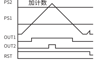
方式8 OUT1:计数值 ≥ SET1 OUT2:计数值 ≥ SET2
