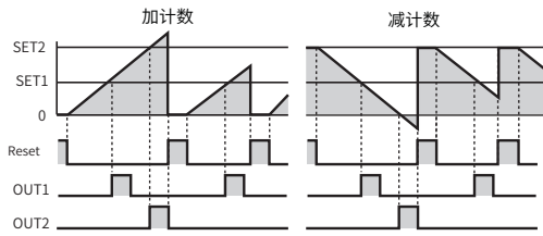
方式5 OUT1:脉冲输出 OUT2:输出保持,计数继续
